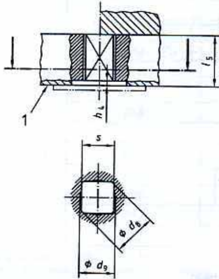
Figure 5 - Drive by parallel square head
