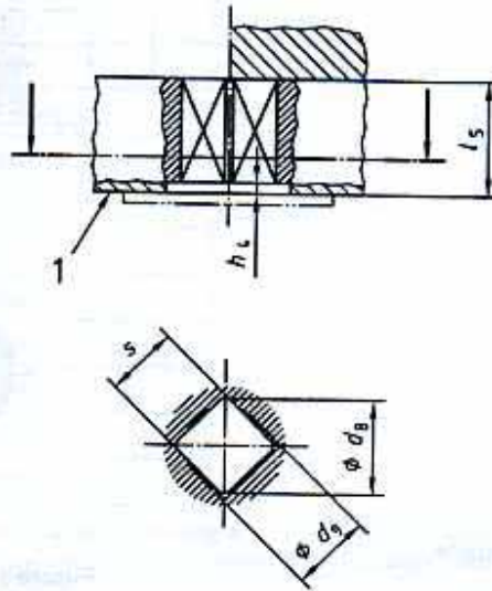
Figure 6 - Drive by diagonal square head
