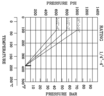
PRESSURE-TEMPERATURE
